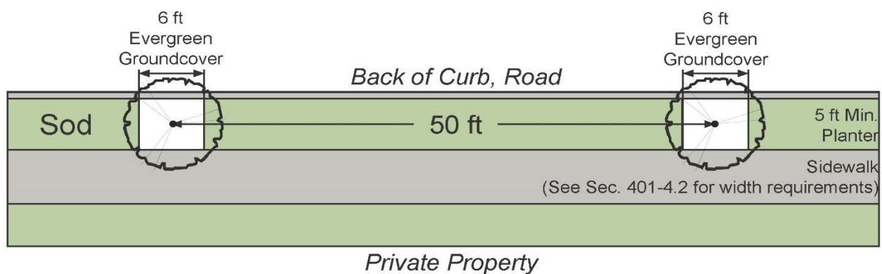
Plan View (above)
