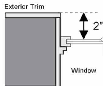
Window Recess with 3.5-inch Trim
